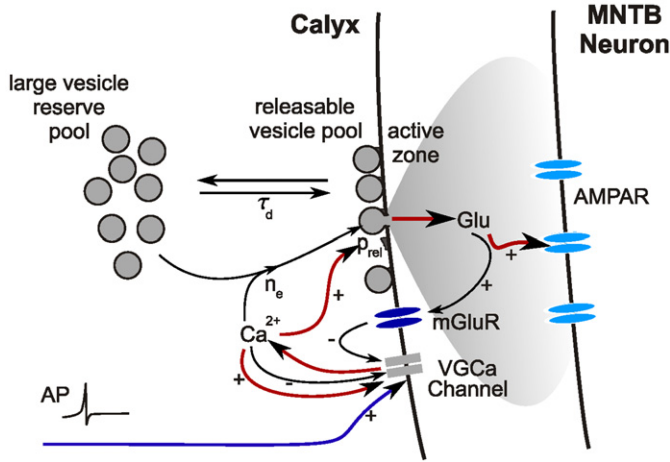
Fig. 1. Schematic illustration of the model. For details, see the main text.
