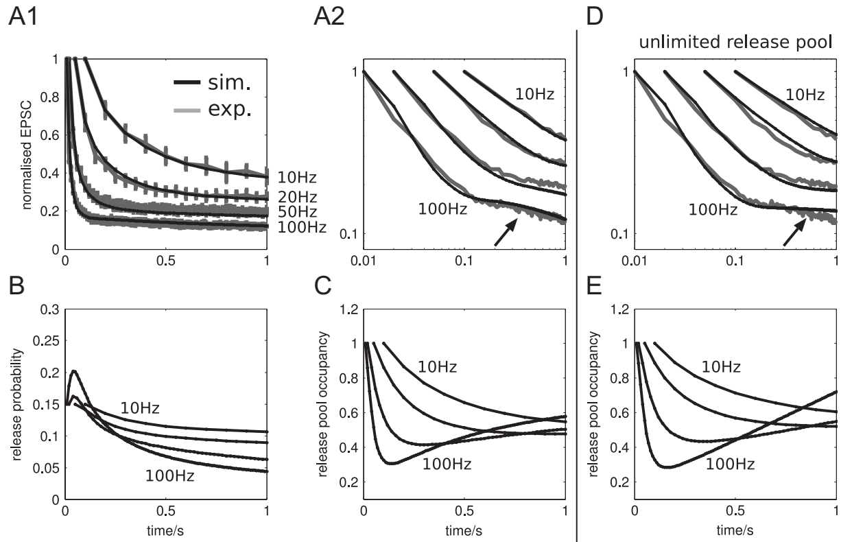
Fig. 2. Simulation of synaptic depression at the calyx of Held during repetitive stimulation at 10, 20, 50 and 100 Hz. (A) Normalised simulated (black) and experimental postsynaptic responses (grey, recorded in rats aged P10–P12; for details on the experimental procedures see [13]), plotted in linear (A1) and double-logarithmic (A2) coordinates. (B) Temporal evolution of the release probability (C) Temporal evolution of the release pool occupancy. (D), (E) as (A2) and (C), but simulated with an unlimited number of release sites. In these simulations, n_e was decreased by factor of 0.6 to fit the experimental data at 10 Hz. Arrows in parts (A2) and (D) indicate the main difference in the behaviour of the two models.
