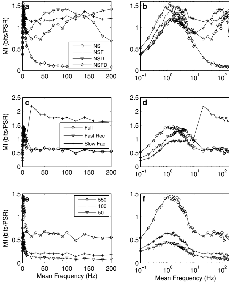
Figure 7: Measures of information transmission for calyx model variants stimulated by Poisson spike trains with mean frequencies ranging from 0.1 Hz to 200 Hz. (a, b) No Slow model with and without facilitation and desensitization (NS: No Slow ; NSF: NS without facilitation; NSD: NS without desensitization; NSFD: NS without both). (c, d) Full model with faster vesicle recycling (Fast Rec: r_p = 2/s ) and slower decay of facilitation (Slow Fac: \tau_f = 0.5 s) (e, f) Full model with different numbers of readily releasable vesicles pools. The mean stimulation frequency is presented as linear (left column) and logarithmic (right column) plots.
